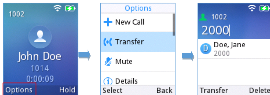
Figure 33: Blind Transfer
