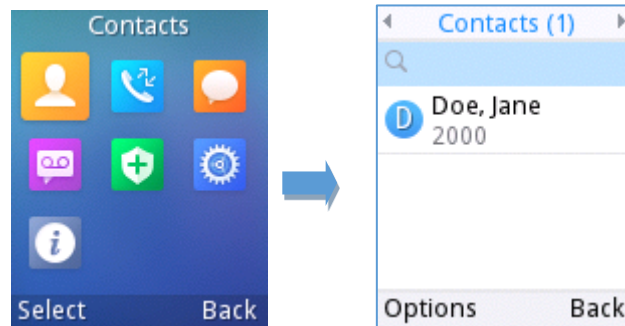
Figure 43: Accessing Contacts
